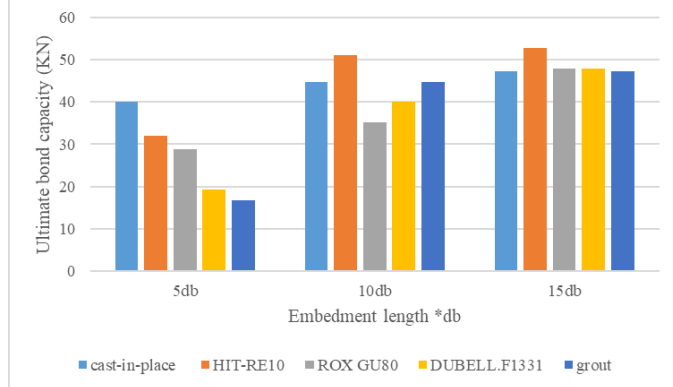
Figure (8) Comparison of the ultimate bond capacity of epoxy brands, grout and cast-in-place with different embedment length for \Phi=10\text{mm}
