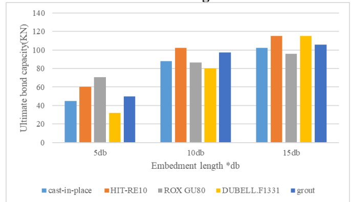
Figure (10) Comparison of the ultimate bond capacity of epoxy brands, grout and cast-in-place with different embedment length for \Phi=16\text{mm}
