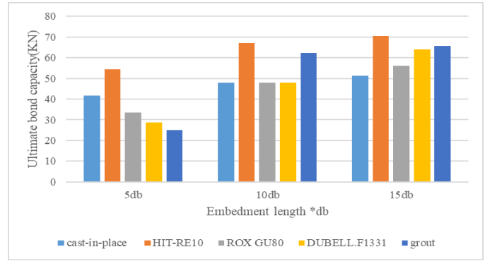
Figure (9) Comparison of the ultimate bond capacity of epoxy brands, grout and cast-in-place with different embedment length for \Phi=12\text{mm}
