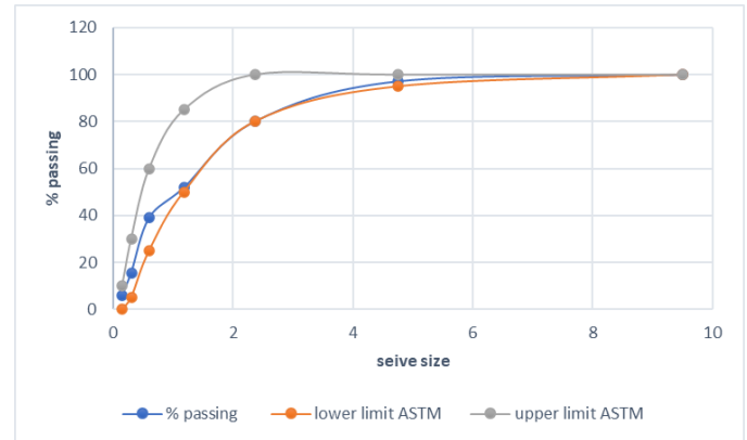
Figure (1) Grading curve of fine aggregate with ASTM limitations
