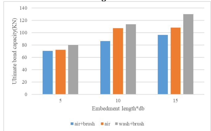
Figure (18) Ultimate bond capacity for adhesive anchor diameter equal to 16mm with different cleaning methods
