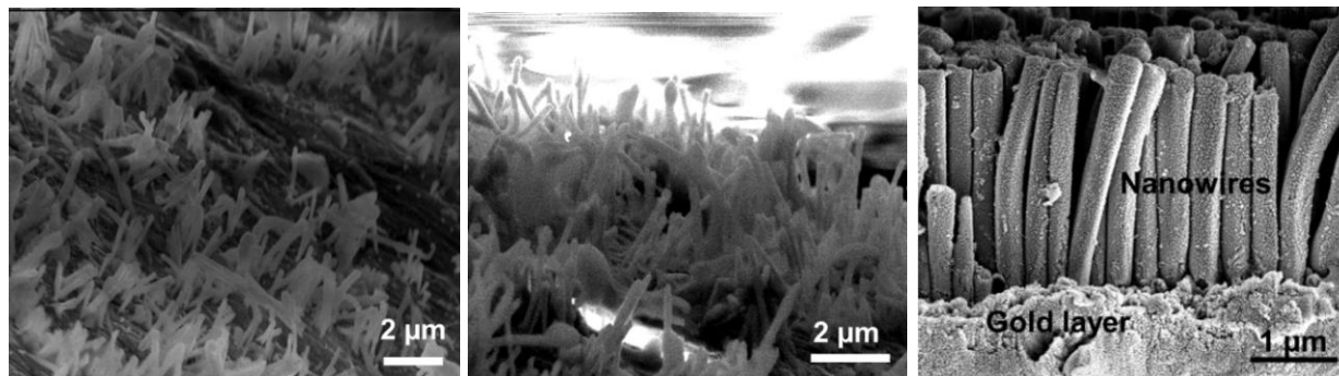
Figure 4 Scanning electron micrographs showing ferromagnetic nanowires bend out and not being released from their base gold layer at a low period of sonication time (2 minutes).
