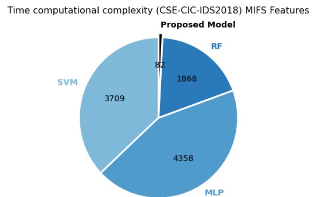
Figure 10: Illustrate time-consuming comparison (MIFS Features)
