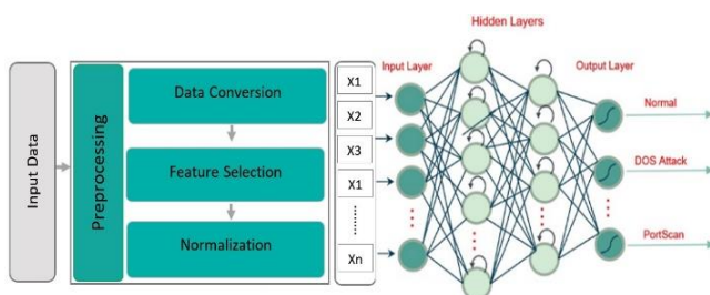
Figure 2: Illustrate the framework of the proposed NIDS model
