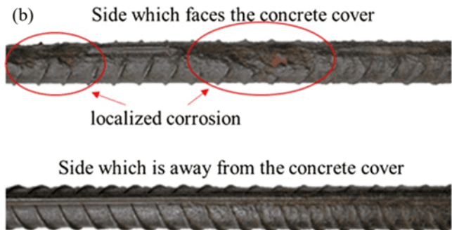
Fig.8. (a) Corrosion distributions of steel reinforcement, typical cross-section of the corroded steel reinforcement (Zhu et al. 2017), (b) a localized corrosion of the bar sides which, faces and away from the concrete cover (Xia et al. 2016).
