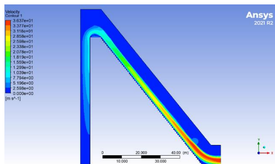
Figure 7: contour of velocity profile.
