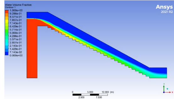
Figure 2: contour of water volume fraction of numerical solution.
