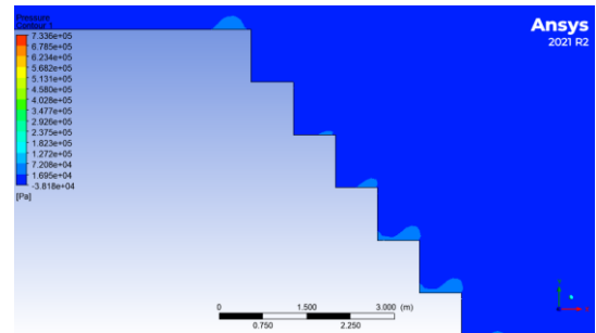
Figure 5: Pressure contour for first steps
