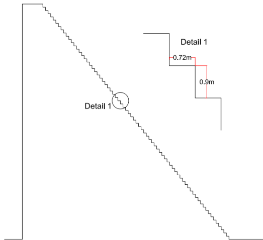
Figure 3: Typical section of Gomaspan dam spillway
